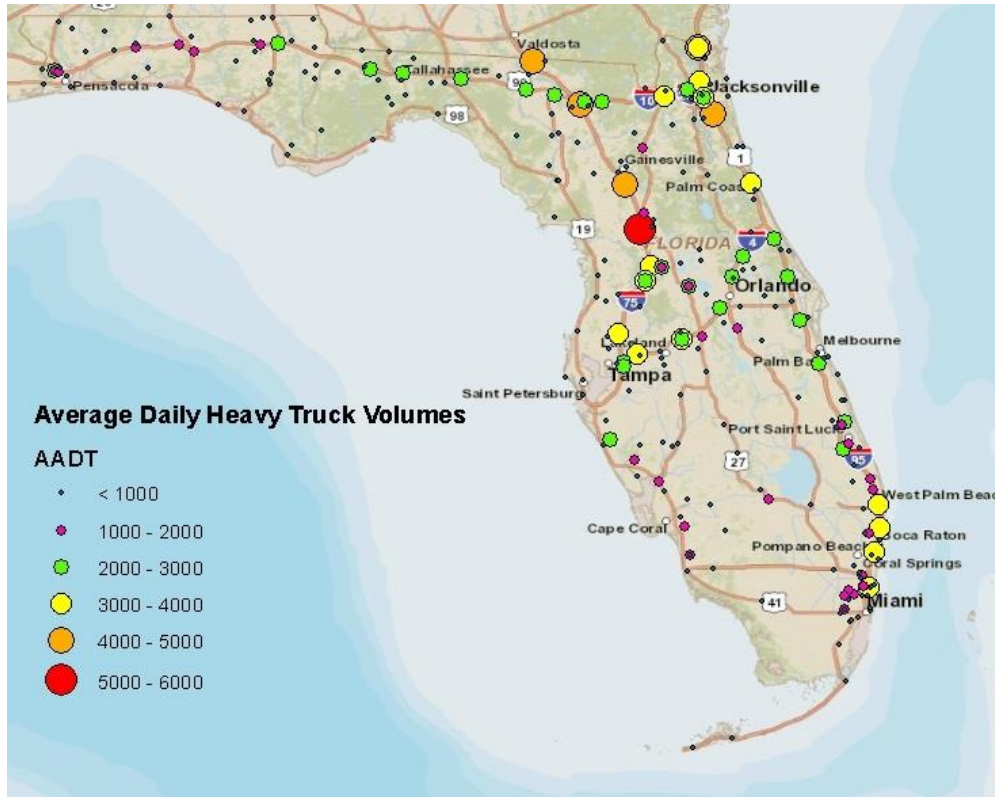
Figure 4.2 Observed Heavy Truck Traffic Flows at Different Telemetric Traffic Counting Sites (TTMS) in Florida
